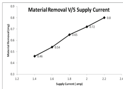
Fig. 5 Effect of supply current on MR
