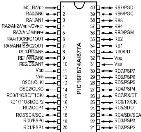
Fig.8 PIC16F874A/877A
