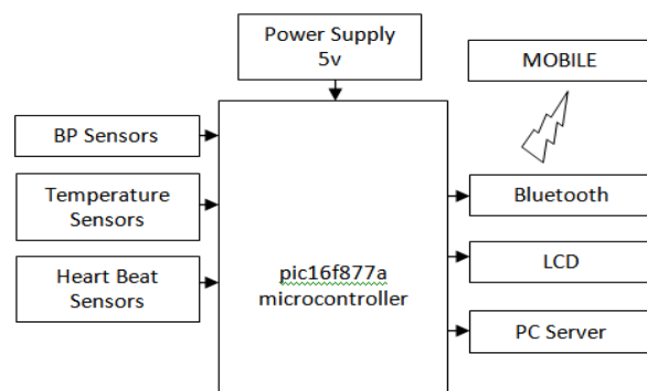
Fig.7 Block diagram of Patient Monitoring System
