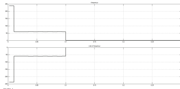
Fig. 8 PMU Frequency and Rate Of Change Of Frequency Measurement Load Side (Before Fault)
