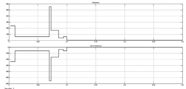
Fig. 12 PMU Frequency and Rate Of Change Of Frequency Measurement Load Side (After Fault)
