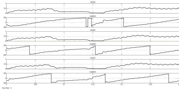
Fig. 10 PMU Current Measurement Load Side (After Fault)
