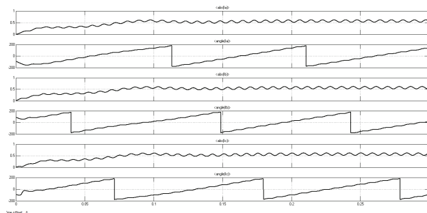
Fig. 6 PMU Current Measurement Load Side (Before Fault
