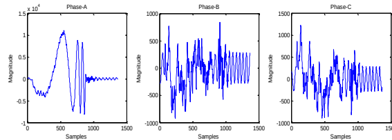
Fig. 8 Approximate-1 coefficient during phase- ‘A-g’ fault at 40% from bus-1
