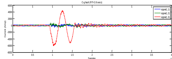
Fig. 15 Three phase current during phase- 'C-g' fault at 50% from bus-1 with FIT=0.04666 seconds
