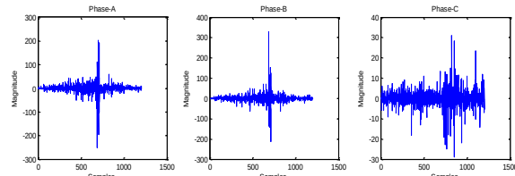
Fig. 5 Detail-1 coefficient during phase- ‘AB-g’ fault
