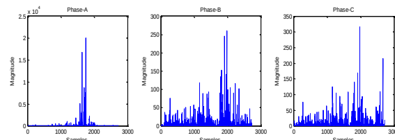
Fig. 10 Squared detail-1 coefficient during phase-‘A-g’ fault at 40% from bus-1
