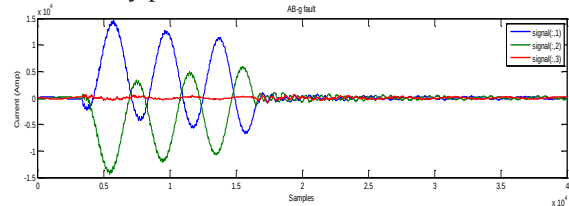
Fig. 3 Three phase current during phase-‘AB-g’ fault at 50% from bus-1
