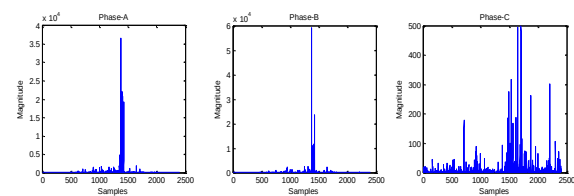
Fig. 6 Squared detail-1 coefficient during phase- ‘AB-g’ fault
