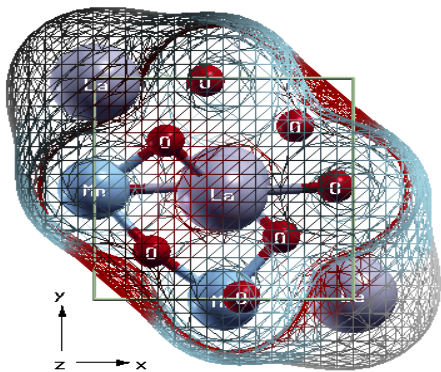
Fig. 2 Molecular surface of Lanthanum manganate crystal as seen along Z-axis
