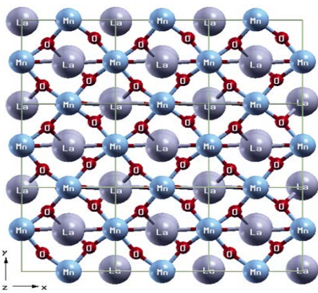
Fig.1 Structure of Lanthanum manganate crystal as seen along Z-axis
